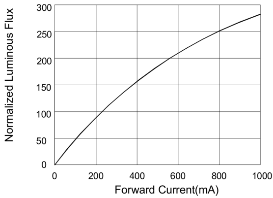
5. Electrical Characteristics Curve
