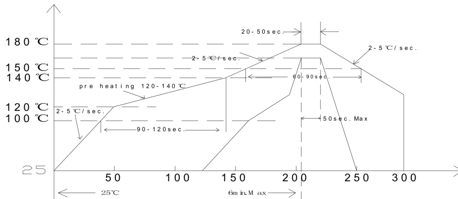
9. Reflow temperature time curve
