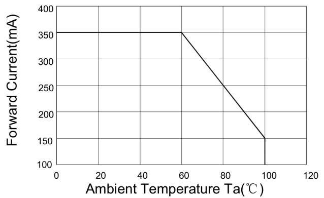
4. Forward Current Derating Curve, Derating based on T_{max}=125^{\circ}C
